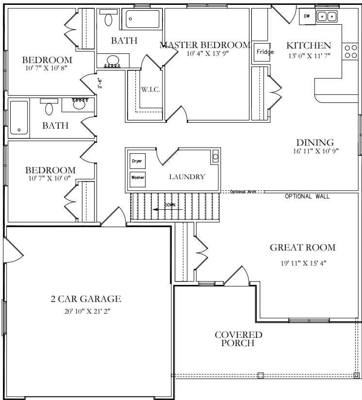
1 Main Floor Plan 21.1 Scale: NTS
