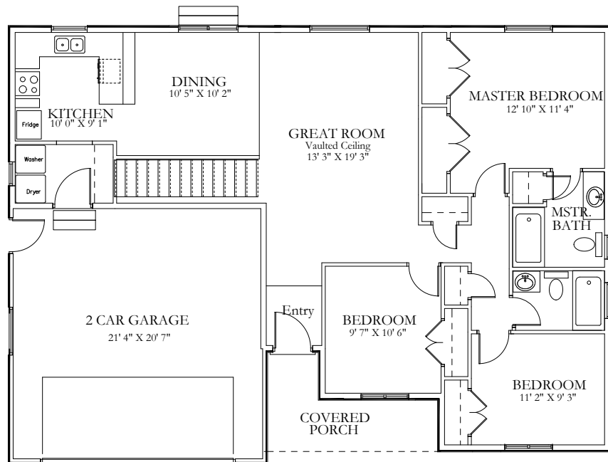
1 Main Floor Plan 21.1 Scale: NTS
