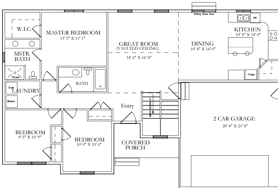
1 Main Floor Plan 21.1 Scale: NTS
